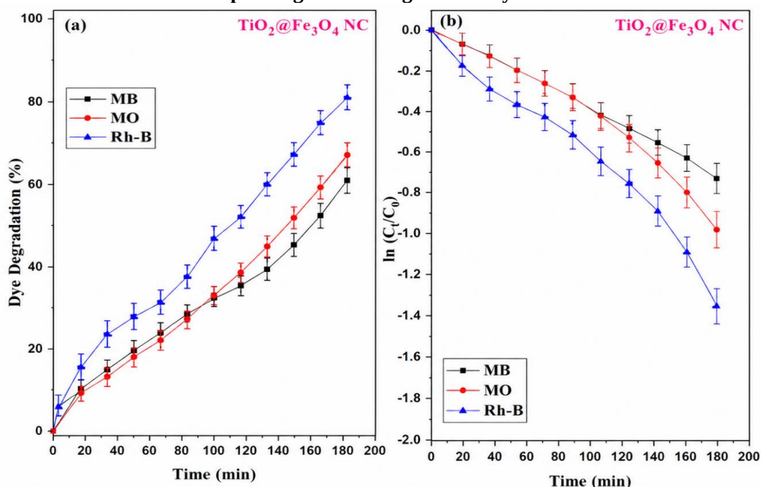
Fig.13. (a) Photocatalytic degradation efficiencies of MB, MO, and RhB over TiO 2 @Fe 3 O 4 nanocomposites under UV-C irradiation, (b) Corresponding pseudo-first-order kinetic plots.
