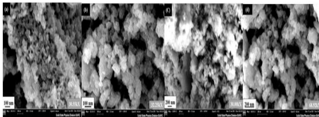
Fig.2: SEM Micrographs of the Synthesized \text{TiO}_2@\text{Fe}_3\text{O}_4 Nanocomposite
