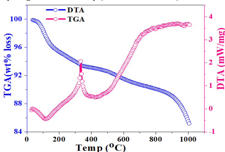
Fig.5: Simultaneous TGA and DTA analysis of the synthesized \text{TiO}_2@\text{Fe}_3\text{O}_4 nanocomposite from room temperature to 1000 °C.
