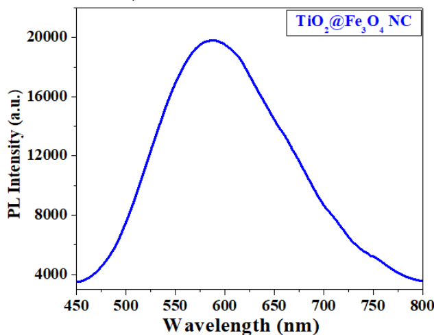
Fig.7: Photoluminescence emission spectrum of the synthesized \text{TiO}_2@\text{Fe}_3\text{O}_4 nanocomposite showing a broad visible emission band centered at about 590 nm.
