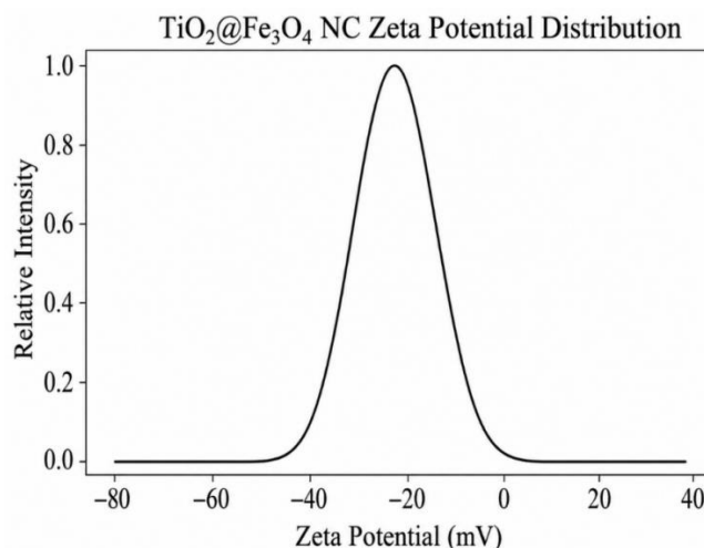
Fig.10: Zeta potential distribution of the synthesized \text{TiO}_2@\text{Fe}_3\text{O}_4 nanocomposite showing a negative surface charge and moderate colloidal stability in aqueous suspension.
