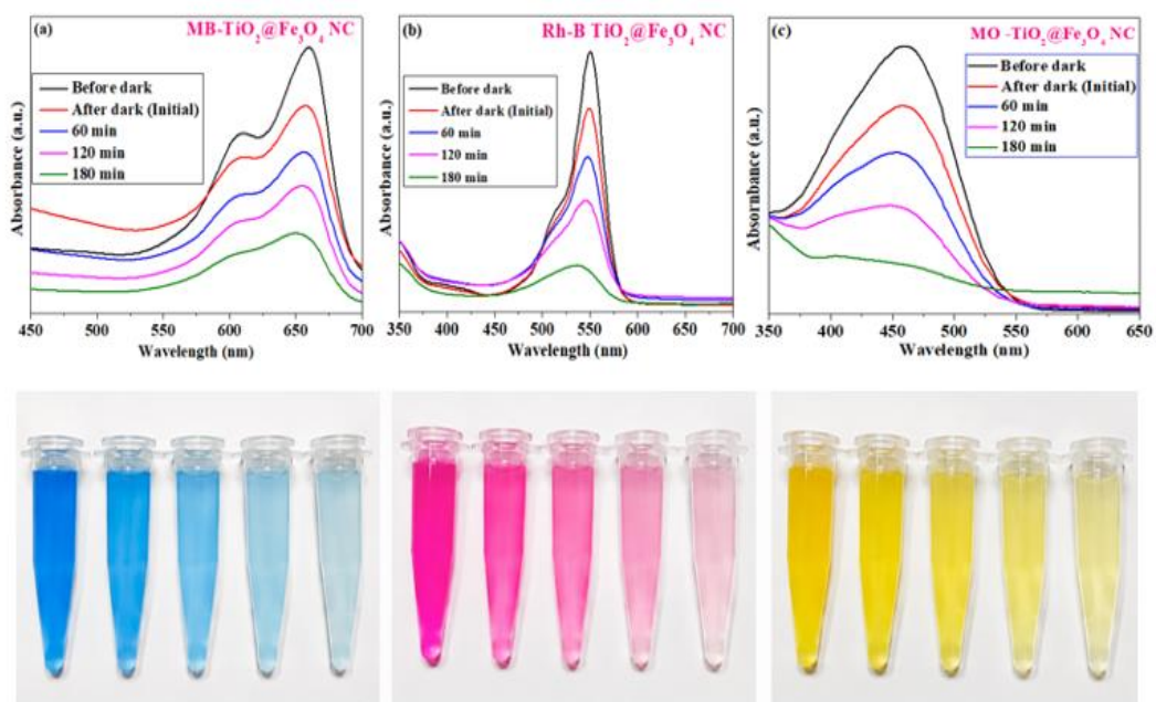
Fig.12: UV-Vis absorption spectra of (a) methylene blue (MB), (b) rhodamine B (RhB), and (c) methyl orange (MO) during photocatalytic degradation over
