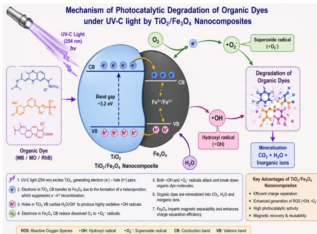
Fig.14: Proposed mechanism of photocatalytic degradation of organic dyes under UV-C irradiation using TiO 2 /Fe 3 O 4 nanocomposites.
