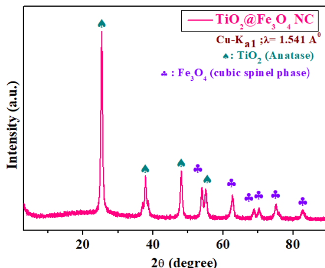
Fig.4: X-ray diffraction pattern of the synthesized \text{TiO}_2@\text{Fe}_3\text{O}_4 nanocomposite showing the characteristic diffraction peaks of crystalline \text{Fe}_3\text{O}_4 and anatase \text{TiO}_2 phases.
