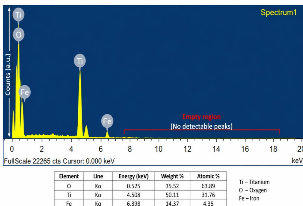
Fig.3: EDX spectrum of the synthesized \text{TiO}_2@\text{Fe}_3\text{O}_4 nanocomposite showing its elemental composition.
