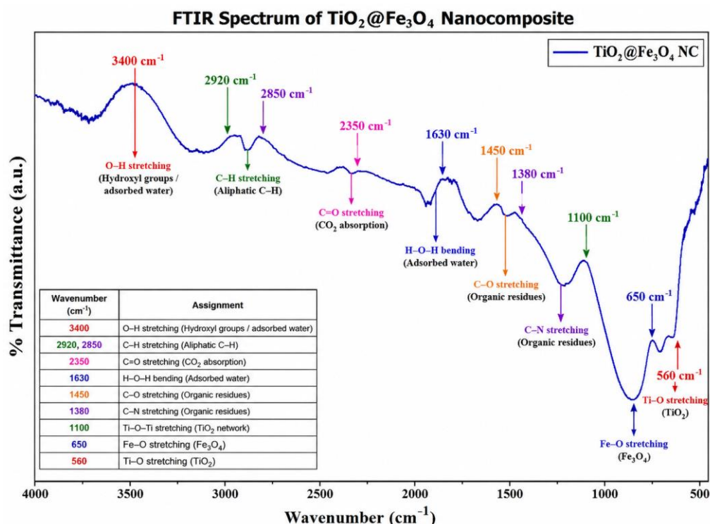
Fig.6: Fourier Transform Infrared (FTIR) spectrum of the synthesized \text{TiO}_2@\text{Fe}_3\text{O}_4 nanocomposite recorded over the wavenumber range of 4000\text{--}500\text{ cm}^{-1} .
