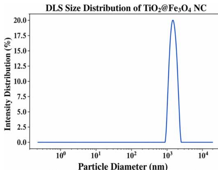
Fig.11: Dynamic Light Scattering (DLS) particle size distribution of the synthesized \text{TiO}_2@\text{Fe}_3\text{O}_4 nanocomposite showing a single dominant hydrodynamic size distribution centered at approximately 1458 nm.
