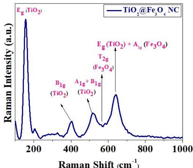
Fig.8: Raman spectrum of the synthesized \text{TiO}_2@\text{Fe}_3\text{O}_4 nanocomposite showing the characteristic vibrational modes of anatase \text{TiO}_2 and cubic spinel \text{Fe}_3\text{O}_4 .
